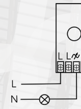
Master Dimmer
