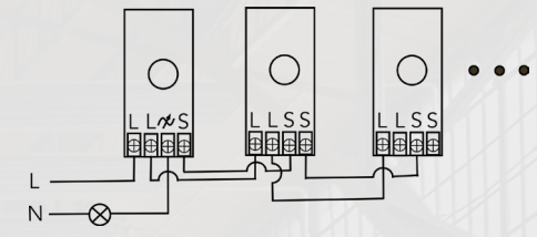
Master Dimmer + 2 Slaves or more
