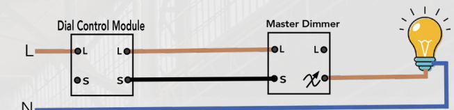
Master Dimmer
