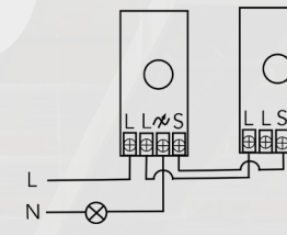
Master Dimmer + 1 Slave
