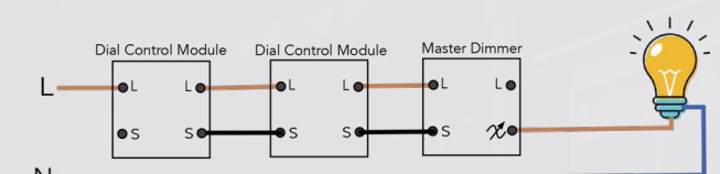
Master Dimmer + 2 Slaves or more
